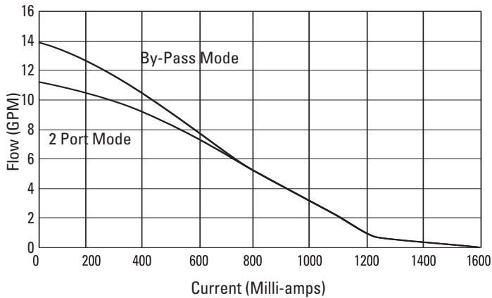
Flow vs Current - A Spool
