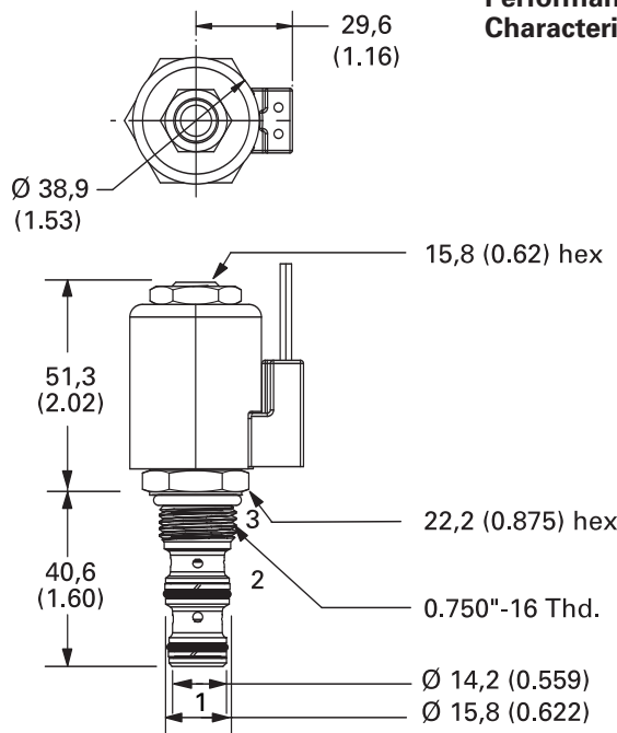
Valve is shown with "N" coil.
