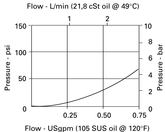
Pressure override, de-energized
